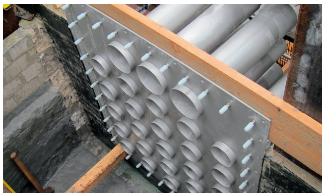
Multiple stainless steel wall sleeve HRD-FUF/o/u
